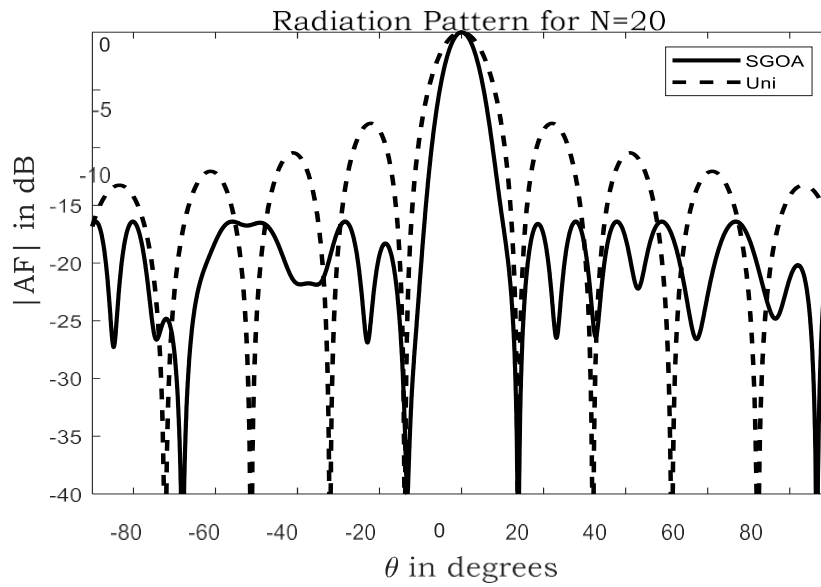
Fig.2. Radiation pattern for N=20
