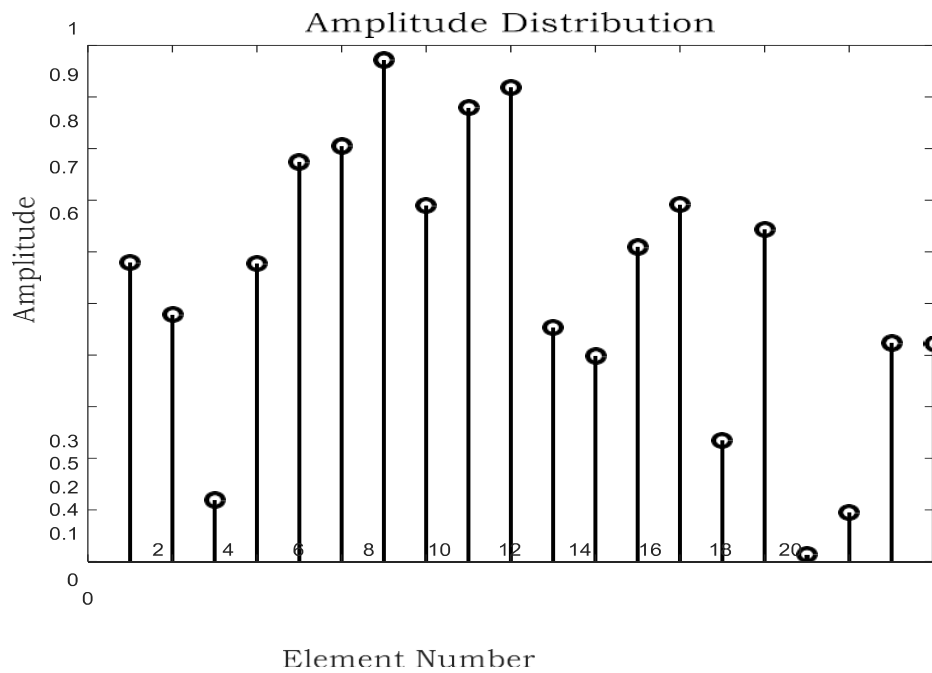
Fig.3. Amplitude distribution for N=20 element circular ar
