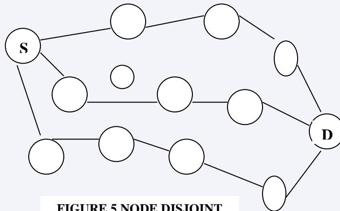
FIGURE 5 NODE DISJOINT
