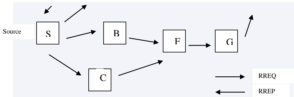
FIGURE 3 BLACK HOLE ATTACK ON AODV
