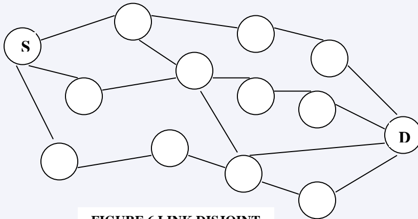
FIGURE 6 LINK DISJOINT
